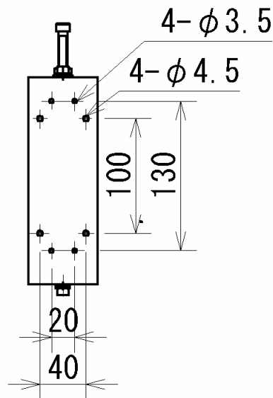
[Force gauge mounting plate]
